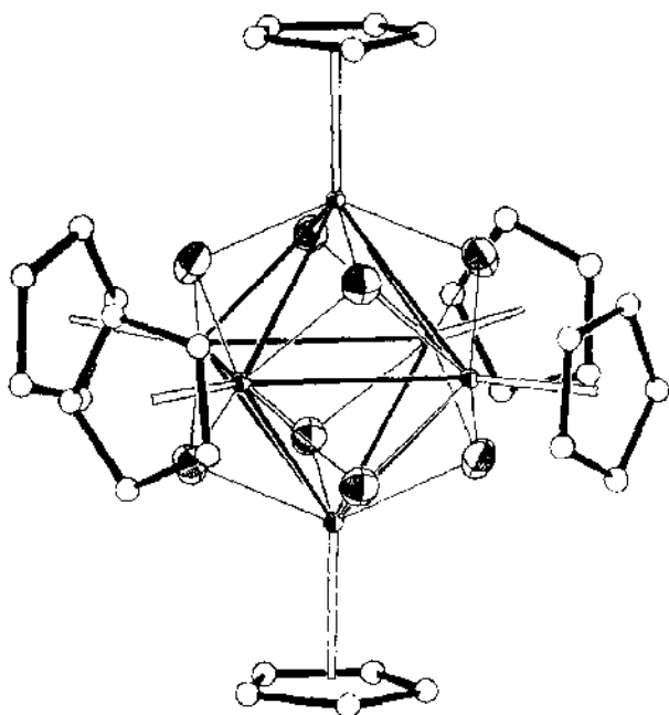
Fig. 4. Structure of [(\eta^5\text{-CpTi})_4\text{O}_8] . Reproduced with permission from ref. 32.
