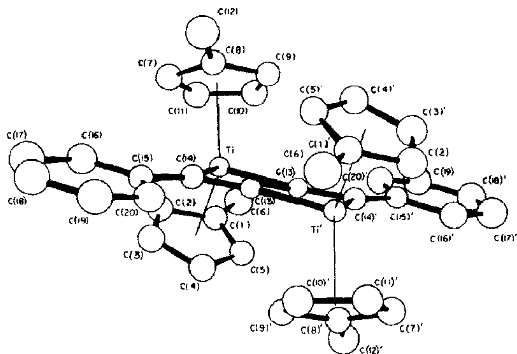
Fig. 8. Structure of \{(\eta^5\text{-CpMe})_2\text{Ti}\}_2(\text{C}_4\text{Ph}_2) . Reproduced with permission from ref. 128.
