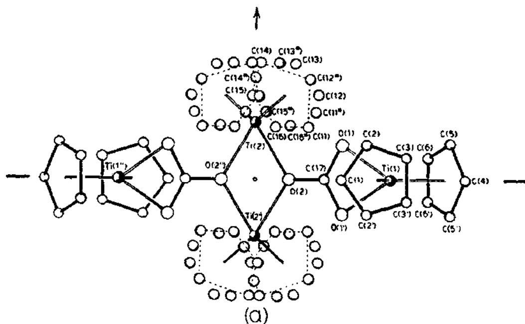
Fig. 10. Structure of \{[(\eta^5\text{-Cp})_2\text{Ti}]_2(\text{CO}_3)_2\} (a) (ref. 133) and of \{[(\eta^5\text{-Cp})_3(\eta^1\text{-}\eta^5\text{-C}_5\text{H}_4)\text{Ti}_2]\{[(\eta^5\text{-Cp})_2(\eta^5\text{-}\eta^5\text{-C}_{10}\text{H}_8)\text{Ti}_2](\mu_3\text{-N}_2)\}\} unit (b) (page 88) (ref. 134). Reproduced with permission.
